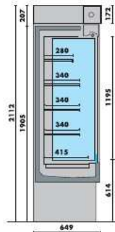
MURAL COM ESTORES ELÉTRICOS ELECTRIC SHUTTER MULTIDECK
