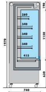
MURAL COM ESTORES MANUAL LP MANUAL SHUTTER MULTIDECK LP
