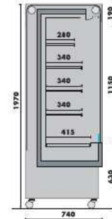
MURAL COM ESTORES MANUAL MANUAL SHUTTER MULTIDECK
