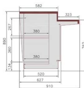
Caisse PMR standard
