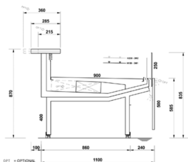
Version libre service
