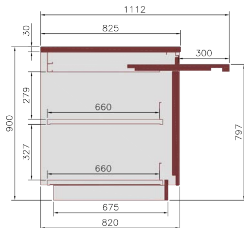
Caisse PMR tablette coulissante
