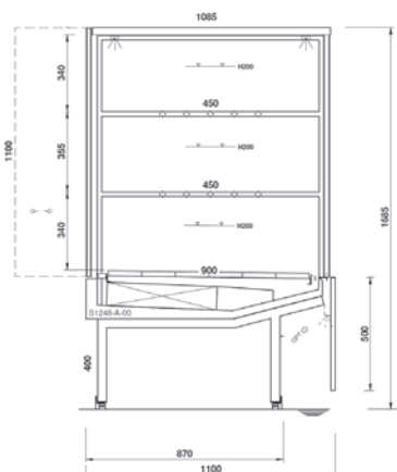
Version tour de maturation
