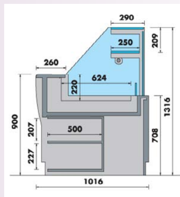
Version Fixe standard
