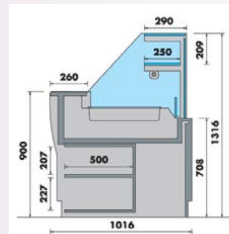
Version cuve inox
